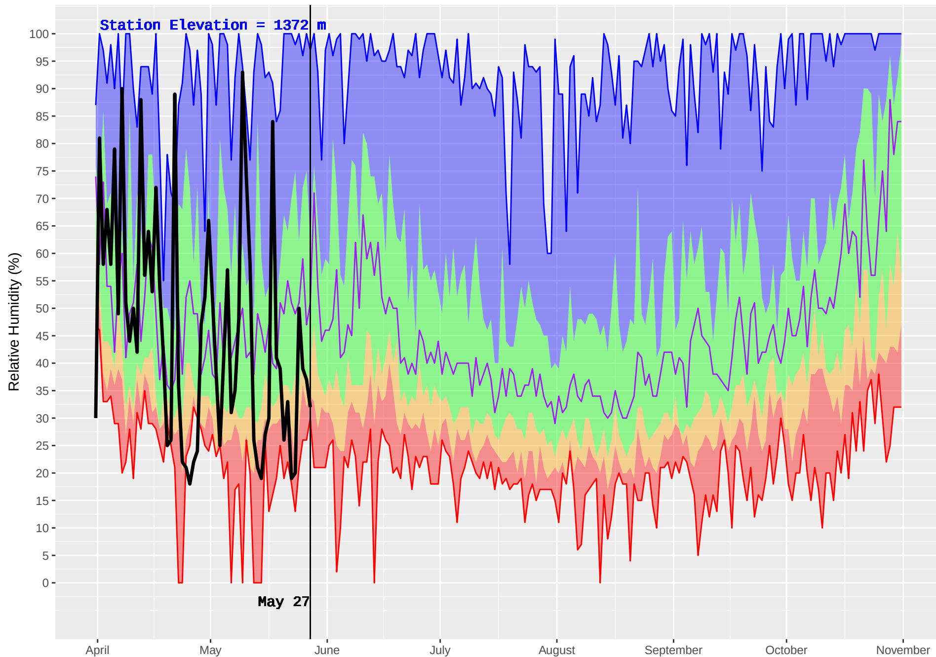
CHERRY LAKE (791) : Historical (1989–2016) and Current (2018) Noon Relative Humidity
