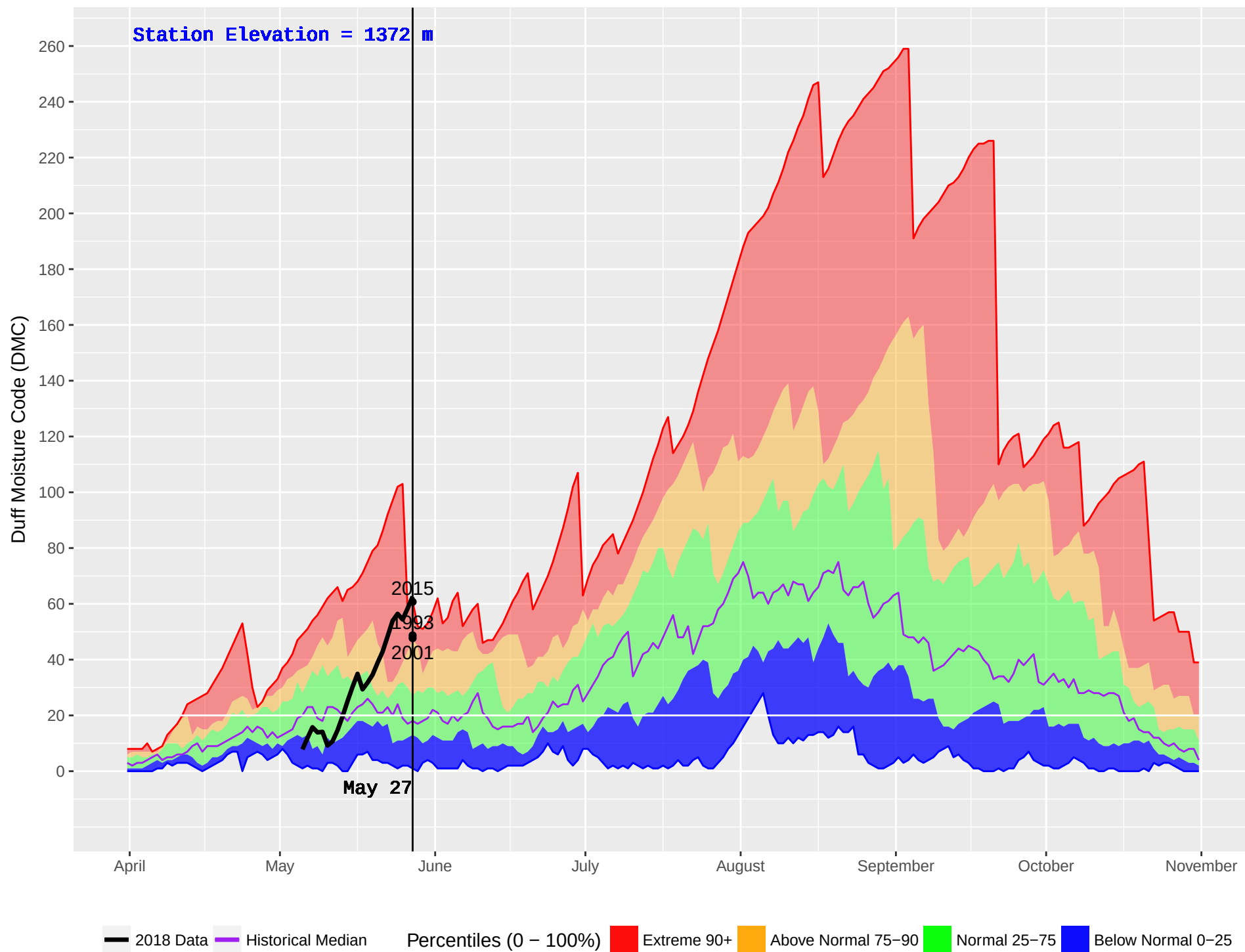
CHERRY LAKE (791) : Historical (1989–2016) and Current (2018) Noon Duff Moisture Code (DMC)
